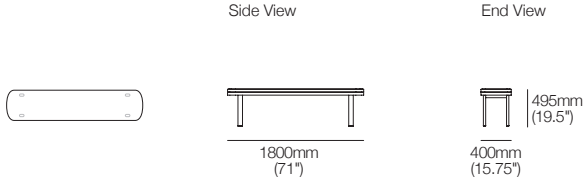
PlateauO Rounded End Dining Bench 1800 Top View
