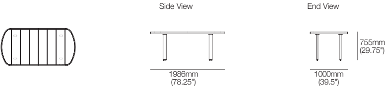
PlateauO Rounded End Dining Table 1986 Top View
