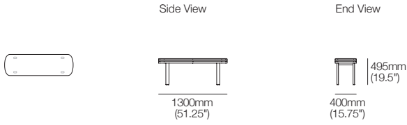
PlateauO Rounded End Dining Bench 1300 Top View
