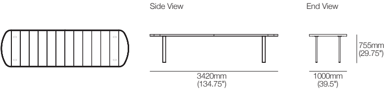
PlateauO Rounded End Dining Table 3420 Top View
