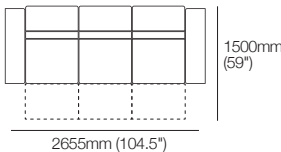
King Cloud Premiere 3-Seater Recliner with Wide Arms 2655mm W | 3-STR 700RW
